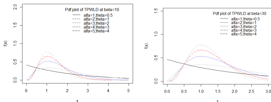
Figure 1. Nature of the p.d.f. of TPWLD for varying values of the parameters
