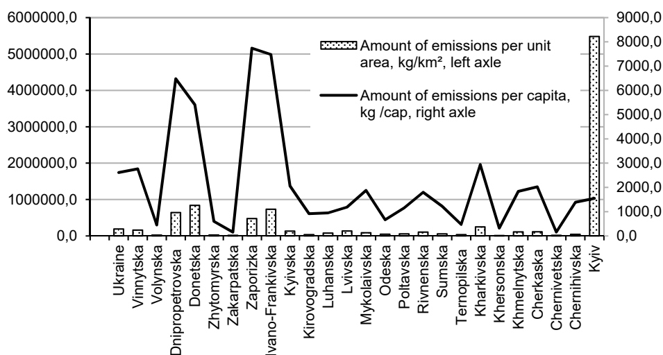
Figure 6. GHG emissions by regions (oblasts) per unit area and per capita, 2020
